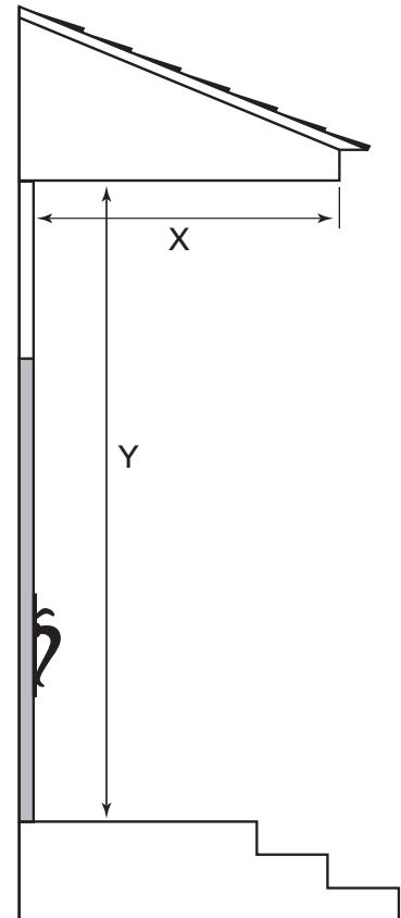
Where X is the length of the overhang required and Y is the distance from the bottom of the door to the base of the overhang.
